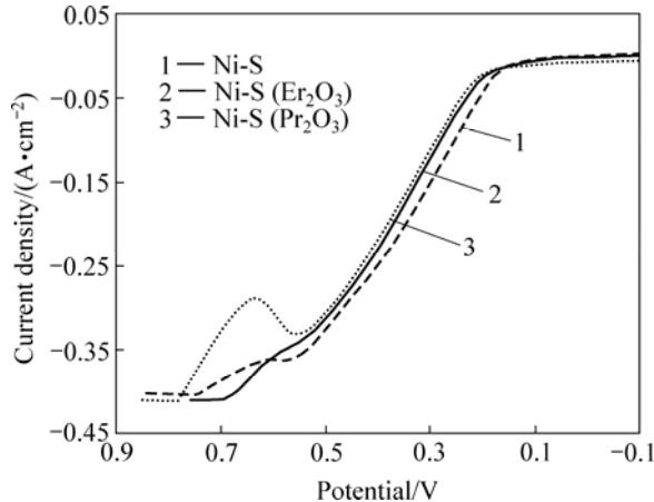
图 3 镀层的阳极极化曲线 Fig.3 Anodic polarization curves of coatings
