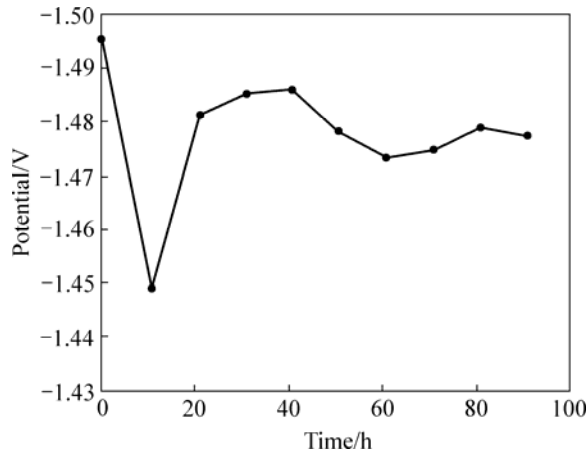
图 4 Ni-S(Pr 2 O 3 ) 电极析氢电位随时间的变化关系 (250 mA/cm 2 ) Fig.4 Relationship between potential and time of Ni-S (Pr 2 O 3 ) electrode under long-term electrolysis (250 mA/cm 2 )
