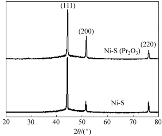
图 6 镀层电极的 XRD 谱 Fig.6 XRD patterns of coating electrodes
