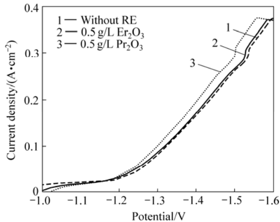
图 2 泡沫镍基 Ni-S 镀层的阴极极化曲线 Fig.2 Cathode polarization curves of Ni-S coatings on foam nickel
