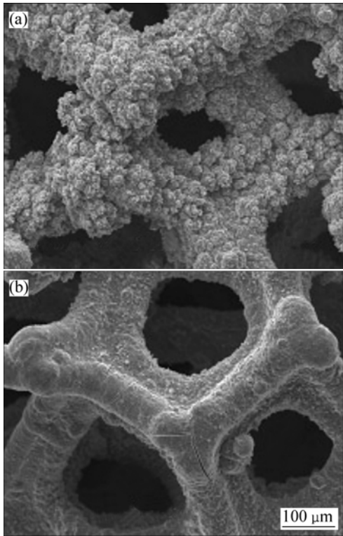
图 5 泡沫镍基 Ni-S 镀层的 SEM 微观结构 Fig.5 SEM micrographs of nickel sulphur coatings on foam nickel substrates with (a) and without Pr 2 O 3 (b)
